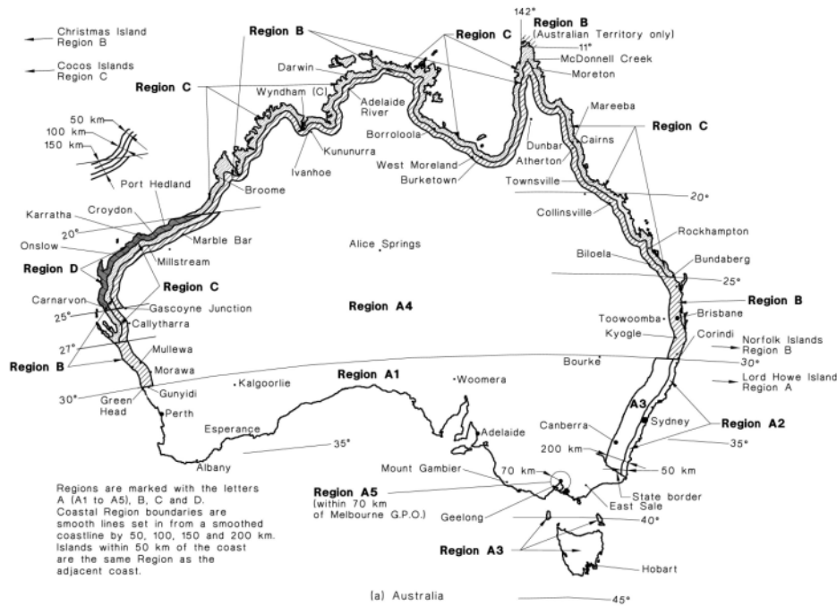
Figure 0.1: Different wind regions in Australia from the Australian Standards AS 1170.2
