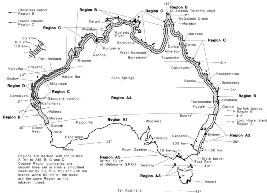
Figure 1: Different wind regions in Australia from the Australian Standards AS 1170.2
