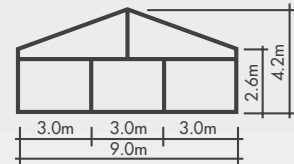
Type: HT9/260
