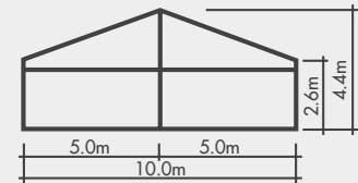
Type: HT10/260
