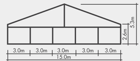
Type: HT15/260
