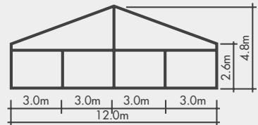
Type: HT12/260
